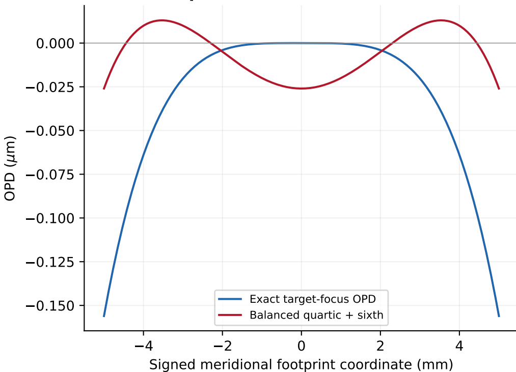
Spherical mirror wavefront
